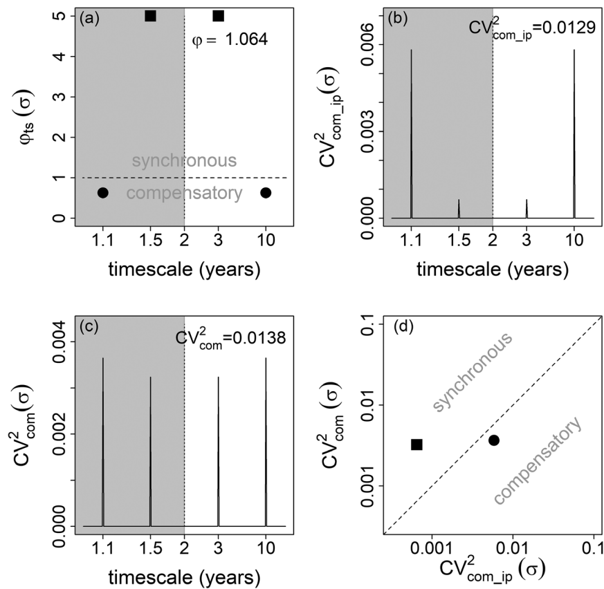
Fig. 3. Application of our theory to the artificial time series of Fig. 1. See text of the Theory section for interpretations. Panels (a–c) show the timescale-specific variance ratio \varphi_{ts}(\sigma) , aggregate population variability CV_{com\_ip}^2(\sigma) , and community variability CV_{com}^2(\sigma) . Timescales less than the Nyquist timescale (gray background) are symmetric to timescales greater than the Nyquist timescale (white background); we present both to reflect the underlying computation of non-timescale-specific quantities (text near top of a–c) as sums or averages across all timescales, both above and below the Nyquist timescale (Theory); but conceptually, we focus on the timescales greater than the Nyquist timescale. The horizontal dashed line (a) indicates the boundary between synchronous and compensatory dynamics for each timescale. Panel (d) compares CV_{com}^2(\sigma) to CV_{com\_ip}^2(\sigma) for the period-3 (square) and period-10 (circle) oscillations; the 1:1 line separates synchronous from compensatory dynamics. For simplicity, the example used sums of sinusoids, which oscillate only at discrete timescales, explaining why plotted quantities are 0 ( CV_{com\_ip}^2(\sigma), CV_{com}^2(\sigma) ) or undefined ( \varphi_{ts}(\sigma) ) except at the timescales of oscillation. Real ecological signals are broadband and should typically yield plots that are well-defined and nonzero at all timescales.
